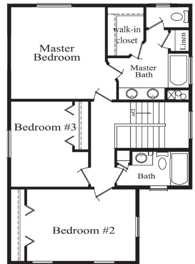
2nd Floor 940 sq. ft.
